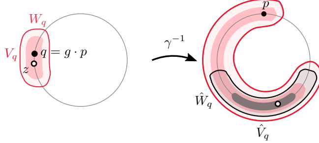
FIGURE 7. The behavior of sets in \partial(\Gamma, \mathcal{H}) described by Lemma 6.8. Given z \in V_q , we pick an element \gamma \in g\Gamma_p so that a uniformly large neighborhood of \gamma^{-1}z is contained in \gamma^{-1}W_q . We cannot pick \gamma^{-1} to expand the metric everywhere close to q —some points in V_q get contracted close to p .
