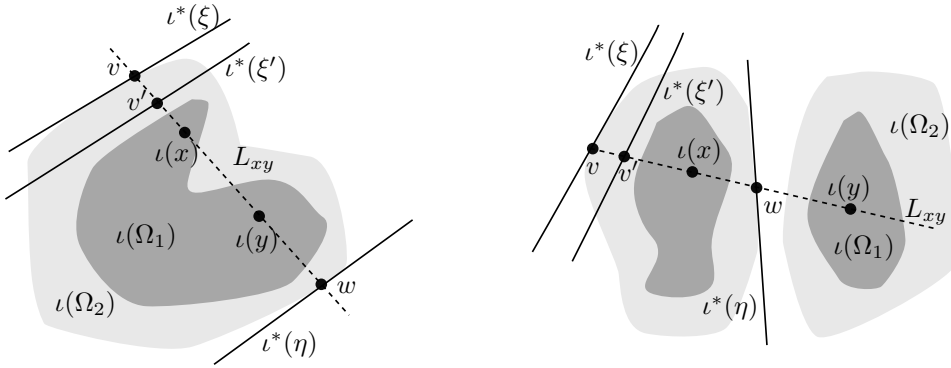
FIGURE 8. We can always find \xi' \in \Omega_1^* close to \xi so that the absolute value of the cross-ratio [\iota^*(\xi), \iota^*(\eta); \iota(x), \iota(y)] increases when we replace \xi with \xi' . In particular this is possible even when the sets \iota(\Omega_1) , \iota(\Omega_2) fail to be convex (left) or even connected (right).
