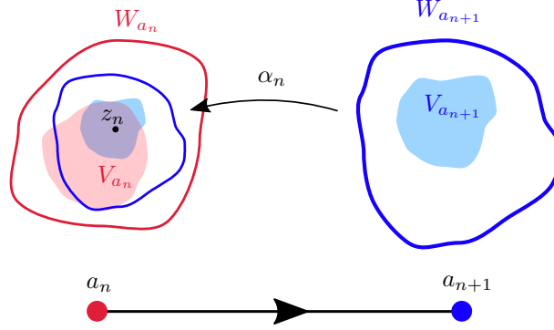
FIGURE 1. Illustration for the proof of Proposition 5.15. The group element \alpha_n nests an \varepsilon -neighborhood of W_{a_{n+1}} inside of W_{a_n} whenever \alpha_n \cdot V_{a_{n+1}} intersects V_{a_n} .
