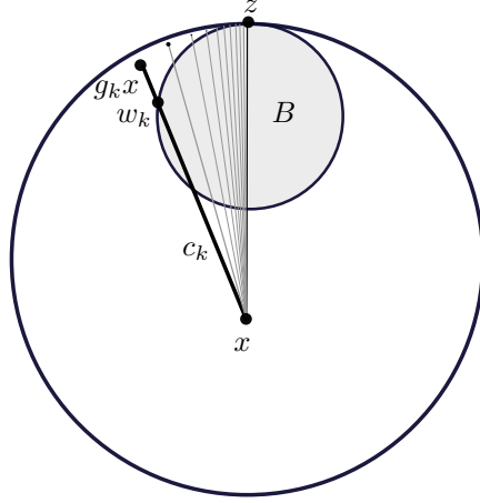
FIGURE 2.1. Illustration for the proof of Lemma 2.17. The geodesic c_k from x to g_k x must enter B , and leave B far from x .
